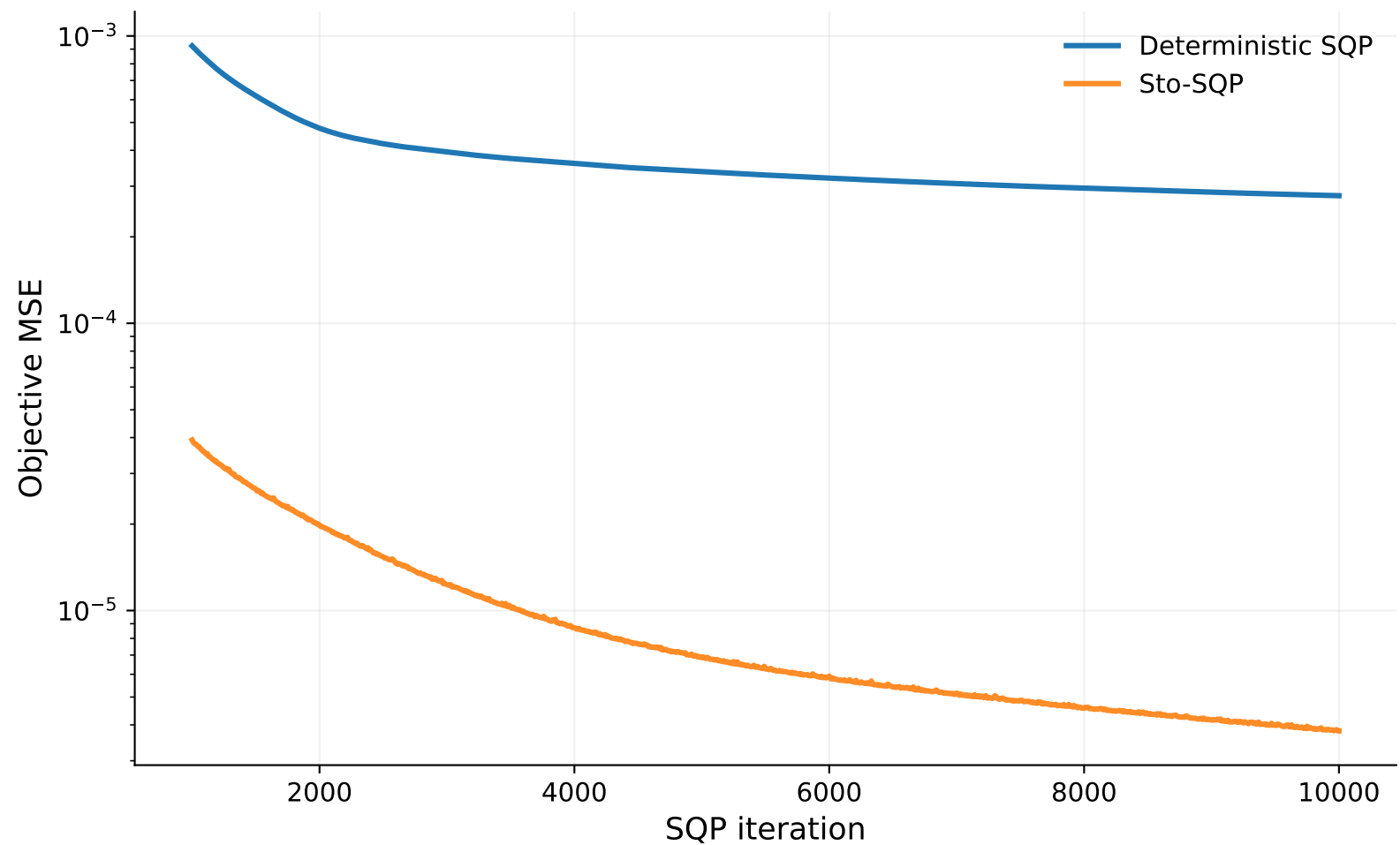
Burgers equation: objective MSE — zoom: iter \geq 1000
