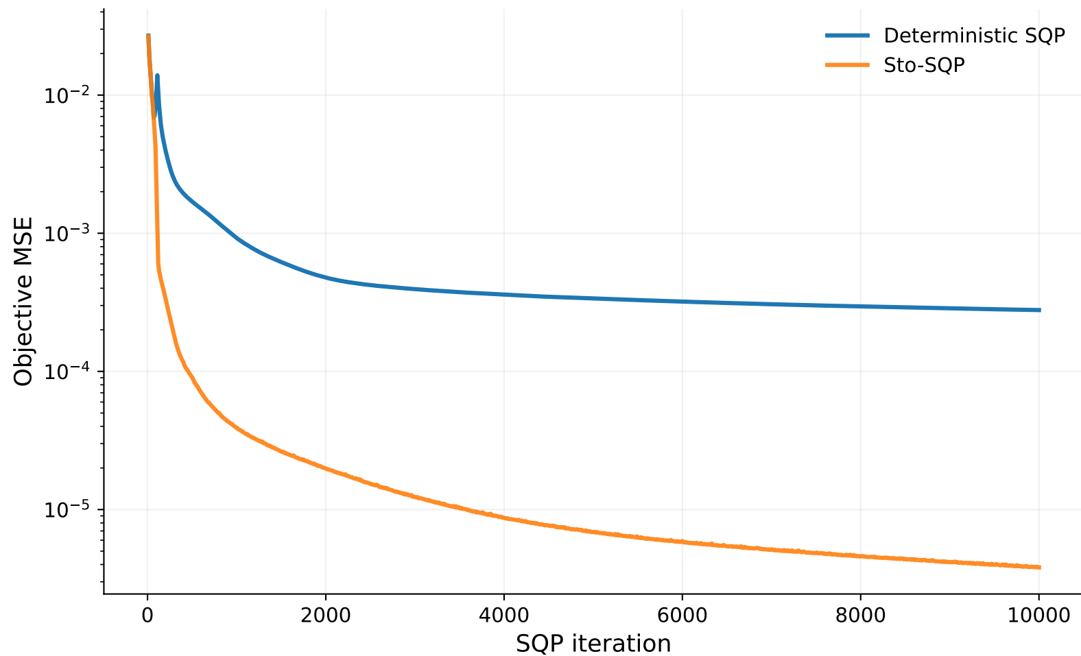
Burgers equation: objective MSE — full trajectory
